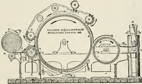
COTTON CARD
